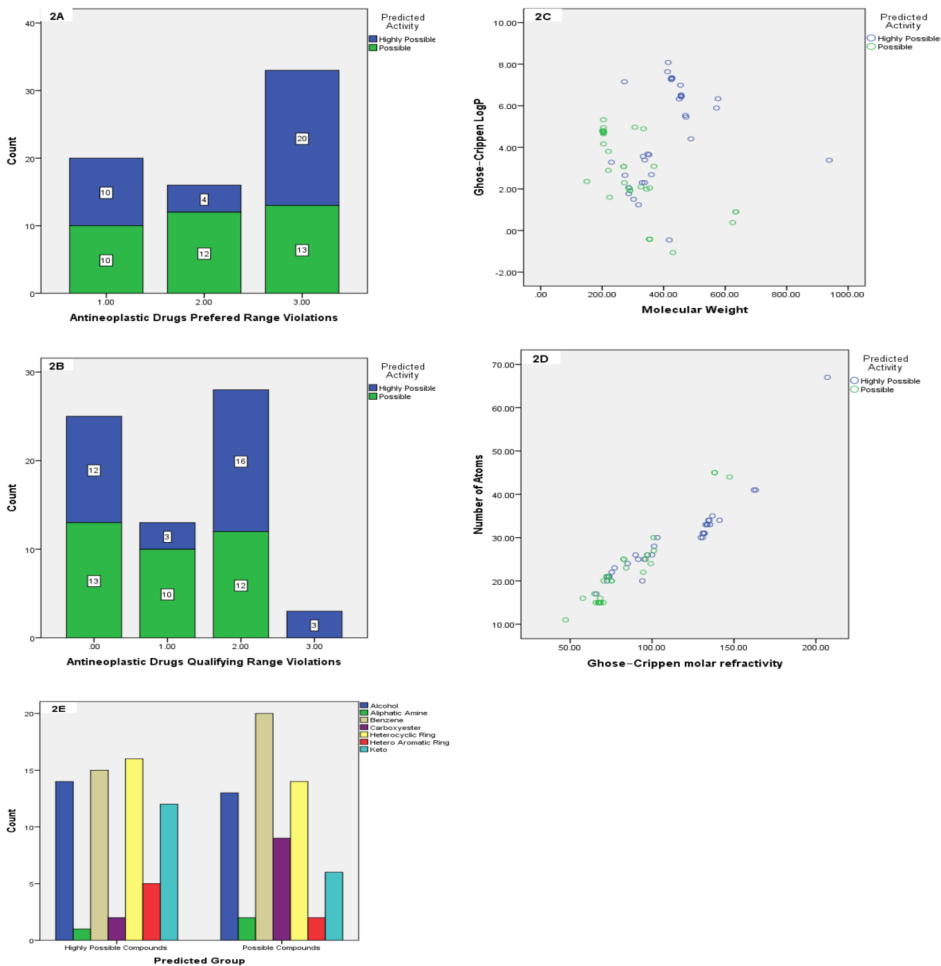
Figure 2: Antineoplastic drug-likeness of predicted phytochemicals according to GVW-indices based ranges. (2A, 2B): Bar graphs of number of violations to the preferred and qualifying antineoplastic drug ranges by predicted phytochemicals. (2C, 2D): Distribution of molecular weight, Ghose-CrippenLogP, Ghose-Crippen molar refractivity and number of atoms ( nA ) of predicted phytochemicals. (2E): Histogram of relevant structural features found in the predicted phytochemicals
