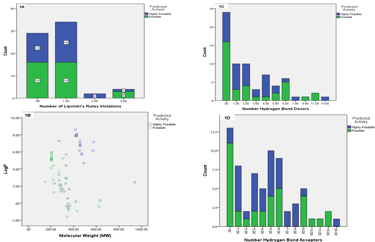
Figure 1: Drug-likeness of predicted phytochemicals based on Lipinski's rule of five (1A): Distribution of predicted phytochemicals based on the number of violations of the rule of five. (1B, 1C, 1D): Distribution of molecular weight, LogP, number of hydrogen bond donors and number of hydrogen bond acceptors of predicted phytochemicals.
